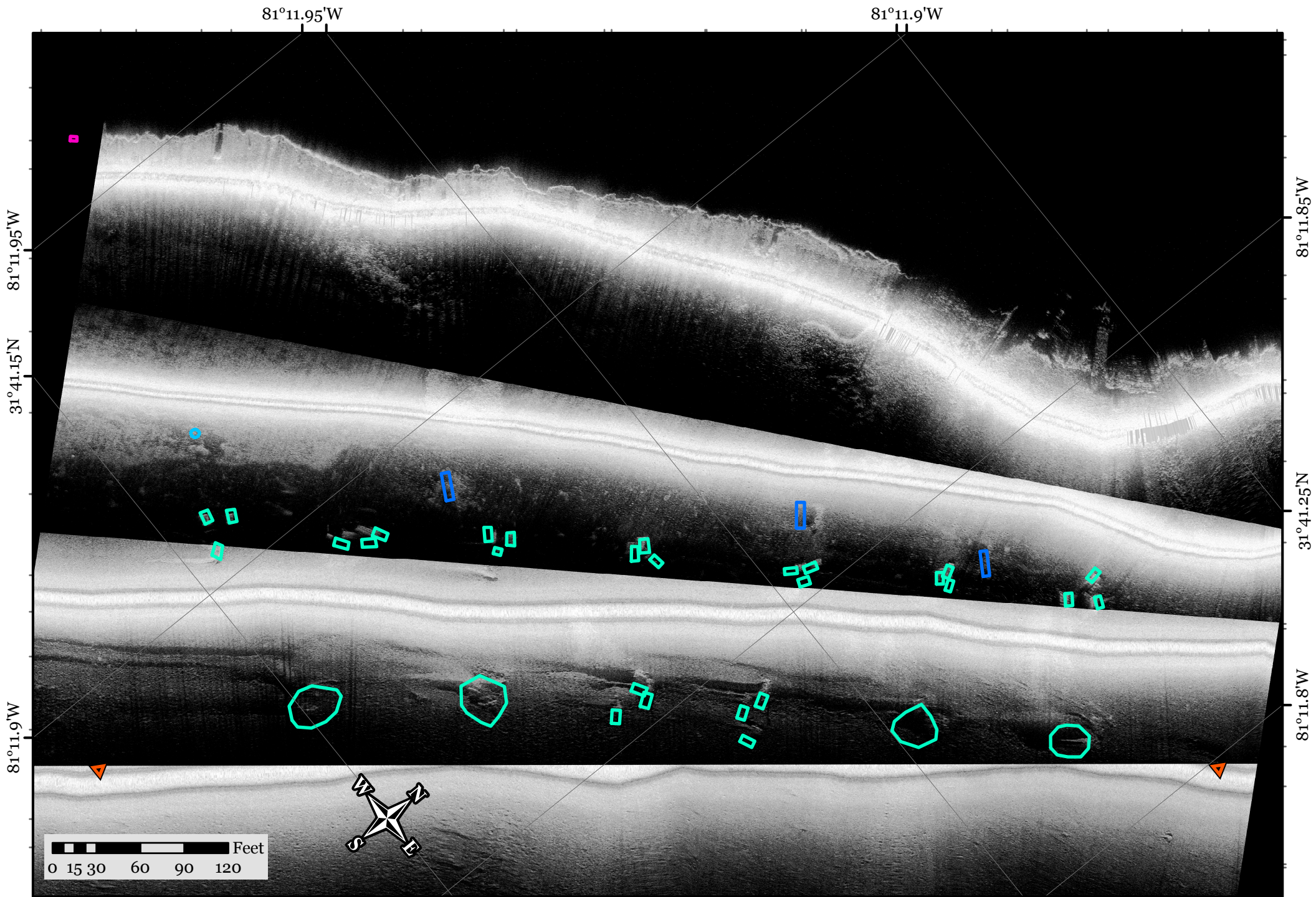
Map of existing structures at Van Dyke Creek inshore artificial reef with side scan sonar imagery taken at high tide on June 29th, 2018.
