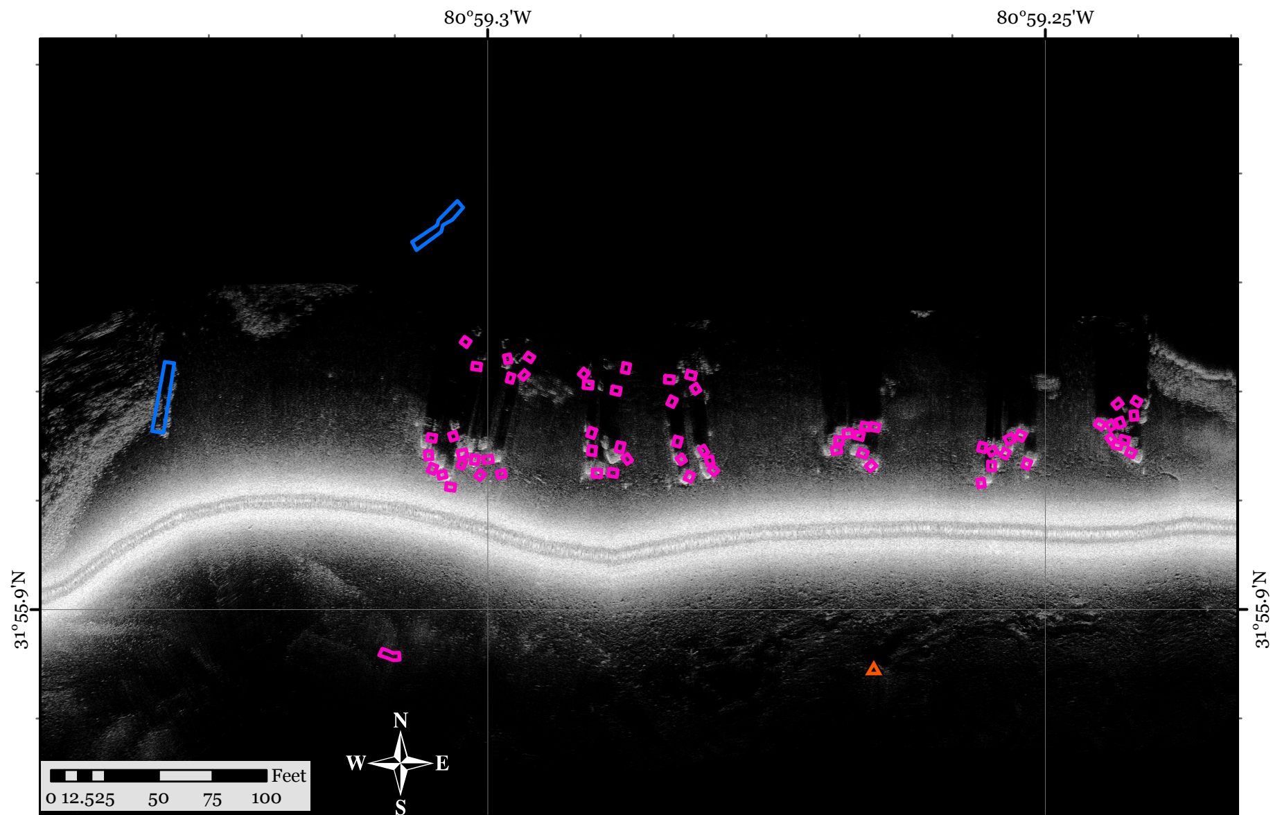
Map of existing structures at Romerly Marsh Creek inshore artificial reef with side scan sonar imagery taken at high tide on June 28th, 2018.
