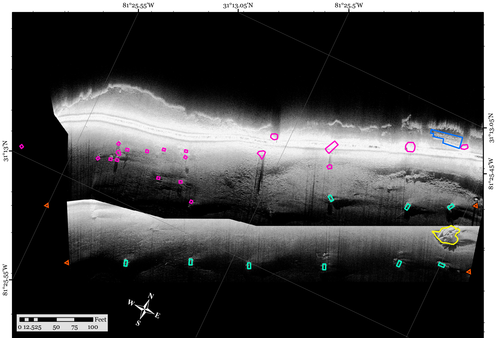
Map of existing structures at Jove Creek inshore artificial reef with side scan sonar imagery taken at high tide on June 14th, 2018.
